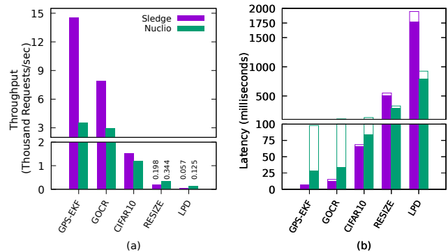
Figure 8. (a) Throughput and (b) Latency of real-world serverless functions at 100 concurrent connections. (Solid bars indicate avg. latencies for 10k iterations, empty bars indicate 99%-tile latencies.)
